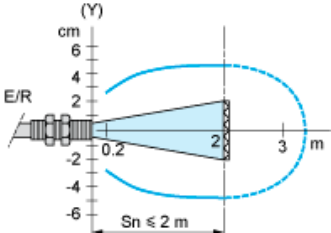
(Y) Ø of beam With reflector XUZC50
